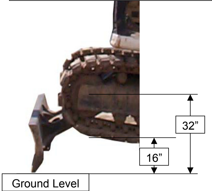
Detail of Blade lowered to lift track
